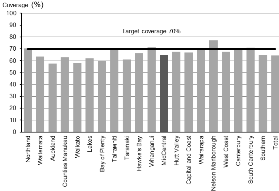
Figure 4: BSA coverage (%) of Pacific women aged 50–69 years in the two years ending 31 March 2017 by District Health Board
